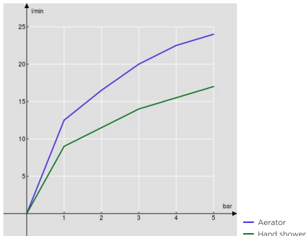
FLOW RATE DIAGRAM: MIXED WATER
