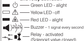
Fig. 5 - "Gas presence alarm" status and relay activation
