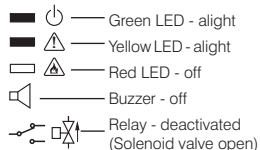
Fig. 2 - "Non operating" status
